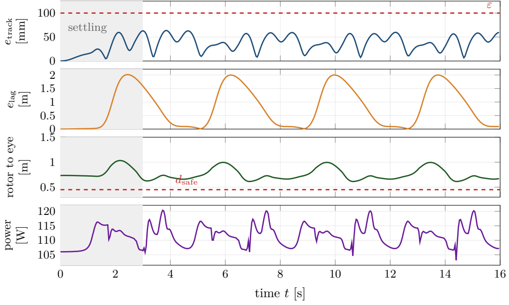
Figure 65: The turnaround flown with the governor. (a) The tracking error against the governed reference stays below the margin \epsilon , which is the hypothesis of proposition 12.11(iv) checked on this run. (b) The lag behind the ideal display position grows to about 2 m at each reversal: the governor lets the display fall behind rather than swing it round the head at the acceleration of fig. 64. (c) The distance from the eye to the nearest rotor disk never approaches d_{\text{safe}} . (d) The electrical power, whose window mean after the settling interval (grey) is the \bar{P} of the energy integral; the brief spikes are the rotor speeds responding to the jerk of the reference at the start and end of each swing.
