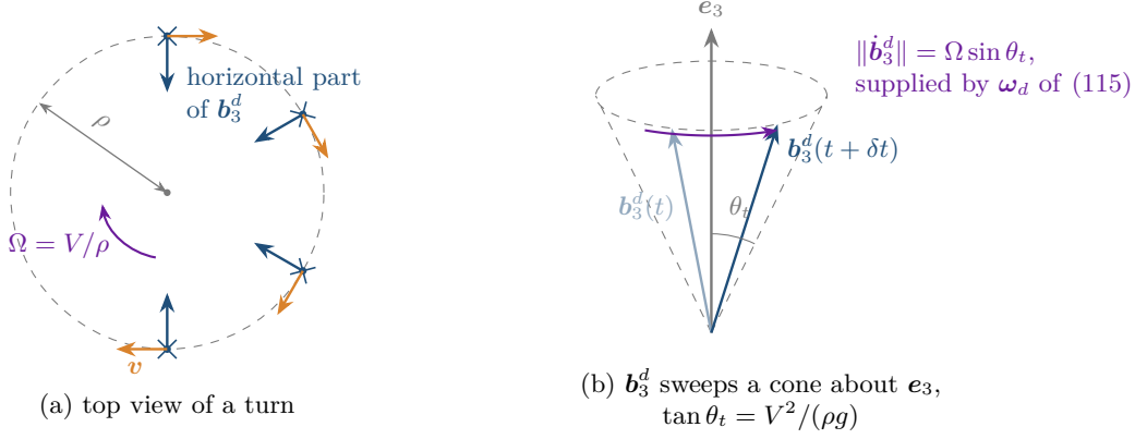
Figure 42: Why a curved path needs angular-rate feedforward. (a) On a turn of radius \rho flown at speed V the commanded force has a horizontal part pointing at the centre of the turn, so the horizontal part of \mathbf{b}_3^d turns with the path at \Omega = V/\rho . (b) \mathbf{b}_3^d therefore sweeps a cone of half-angle \theta_t about \mathbf{e}_3 , with \tan \theta_t = V^2/(\rho g) , and changes at the rate \Omega \sin \theta_t even in a perfectly steady turn. With \boldsymbol{\omega}_d = 0 the attitude loop sees that rate as a persistent error and settles at a lag of about K_\omega \|\boldsymbol{\omega}_d\|/K_R ; eq. (115) supplies the rate instead.
