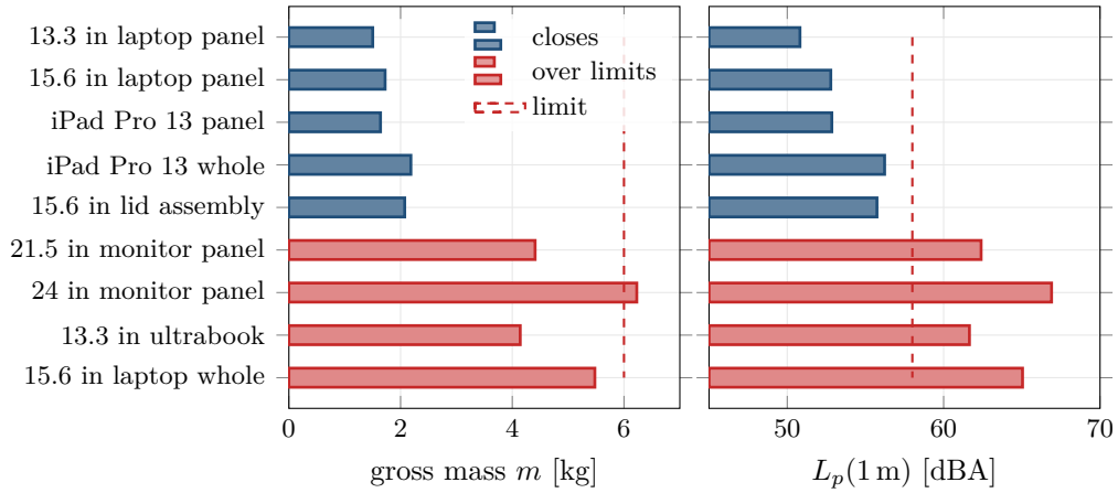
Figure 59: The display candidates of table 6, each with its aircraft re-optimised. Left: gross mass, against the 6.0 kg limit. Right: free-field level at 1 m, against the 58 dBA limit. Every candidate that fails exceeds the noise limit, and only one of them exceeds the mass limit: a heavier display needs a more heavily loaded rotor, and by observation 9.3 that is paid for in decibels long before it is paid for in kilograms.
