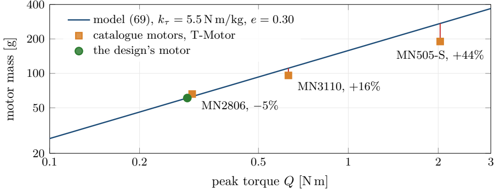
Figure 58: The calibrated motor-mass model eq. (69) against catalogue motors, on logarithmic axes on which the model is a straight line of slope 1/(1+e) = 0.77 . The red connectors are the model errors of table 5: small at the size of motor this design uses (the green point, the design’s 61 g motor at its torque for maximum thrust) and conservative at the large end.
