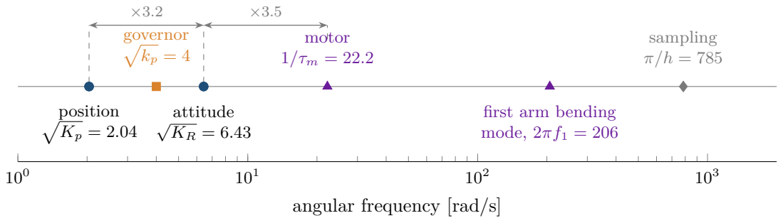
Figure 44: The frequency ladder of the design’s cascade on a logarithmic axis. Each loop is at least a factor of three slower than the one it relies on: position at \sqrt{K_p} , attitude at \sqrt{K_R} , the motors at 1/\tau_m . The governor’s filter at \sqrt{k_p} shapes the reference and closes no loop on the vehicle. The first bending mode of the arms and the sampling rate of the controller lie one and two orders of magnitude above the fastest loop, which is the condition under which the airframe may be treated as rigid and the sampled controller as continuous.
