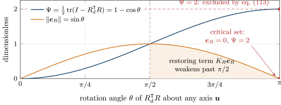
Figure 41: The attitude error for a rotation of R_d^T R by the angle \theta about any unit axis \mathbf{u} , for which \text{tr}(R_d^T R) = 1 + 2 \cos \theta gives \Psi = 1 - \cos \theta and \mathbf{e}_R = \sin \theta \mathbf{u} . The configuration error grows monotonically to its maximum 2 at \theta = \pi , but the restoring term, proportional to \mathbf{e}_R , peaks at \pi/2 and decays to zero at \pi (shaded). Every rotation by \pi is therefore a critical point of \Psi at which the proportional feedback vanishes, which is why eq. (113) excludes \Psi = 2 and why no continuous feedback of this kind is global on \text{SO}(3) .
