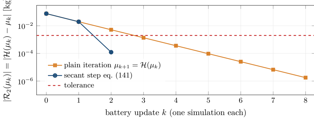
Figure 54: Convergence of the battery loop on the pacing mission, flown with an 8s window so that plain iteration can be run to eight updates at reasonable cost. Plain iteration \mu_{k+1} = \mathcal{H}(\mu_k) contracts linearly, the residual falling by a factor of about 0.263 per update, which is \mathcal{H}' of proposition 13.6 at this design. The guarded secant step eq. (141) takes the same first step and is below the tolerance on the third update. Each point costs one full simulation.
