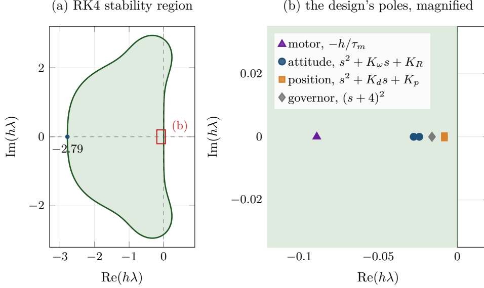
Figure 55: (a) The stability region of classical RK4, \{z : |1 + z + z^2/2 + z^3/6 + z^4/24| \leq 1\} , which reaches -2.79 on the negative real axis. (b) The products h\lambda for the poles of the design's loops at h = 4 ms: the motor lag, the attitude loop s^2 + K_\omega s + K_R , the position loop s^2 + K_d s + K_p and the governor's filter. The fastest, the motor, sits at h\lambda = -0.0889 , about thirty times inside the boundary, so the step is set by accuracy and by the sampling of the controller, not by stability.
