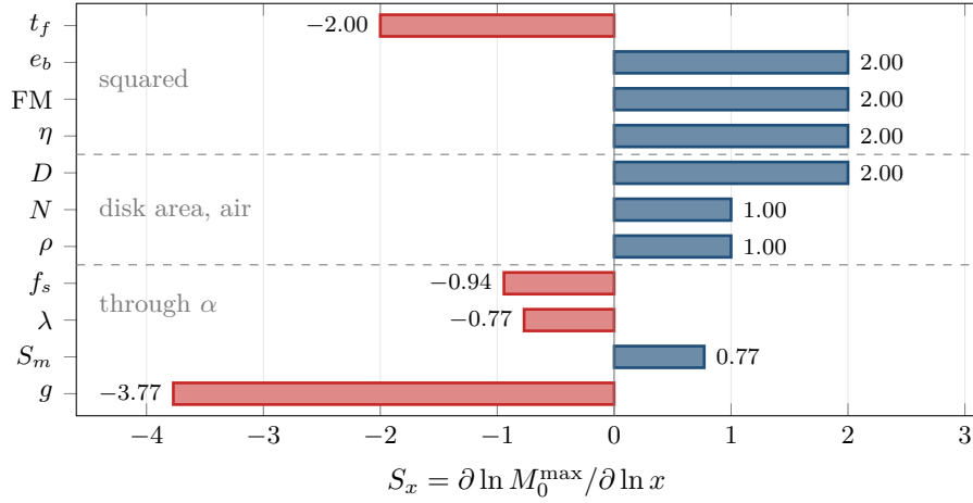
Figure 19: Logarithmic sensitivities of M_0^{\max} at the engine’s default parameters, computed by central differences in \ln -space. The top group are the squared levers of eq. (54); the middle group are disk area, entering as D^2 and N , and air density, eq. (55); the bottom group act through \alpha and are eq. (56), here with \gamma_m/\alpha = 0.257 . Every bar agrees with theorem 7.3 to three decimals. A bar of length two means a 10 % change in the parameter moves the critical load by about 20 %.
