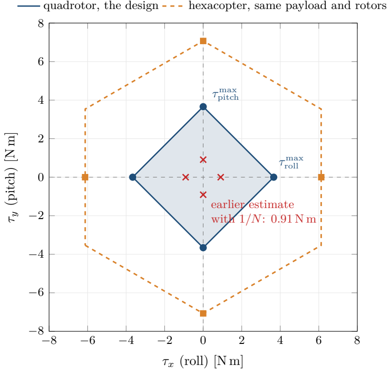
Figure 43: Attainable torque sets in the roll and pitch plane with thrust held at mg and the yaw moment at zero, computed from the engine through their support function: one linear program of the form eq. (116) for each of 240 directions. The quadrotor’s set is a square turned by 45^\circ whose axis intercepts are \tau_{\text{roll}}^{\max} = \tau_{\text{pitch}}^{\max} = 3.66 \text{ N m} , the balanced differential of eq. (117); the crosses mark the earlier estimate with the factor 1/N , a quarter of it. The hexacopter carrying the same payload on the same rotors (gross 2.565 \text{ kg} ) has a hexagonal set that reaches further in pitch than in roll: its roll differential also produces a yaw moment, which the zero-yaw constraint must cancel, while its pitch differential does not. Its authority in the sense of eq. (116) is the smaller intercept, roll.
